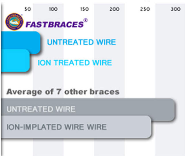
Frictional Resistance to Motion (Grams of Force)
